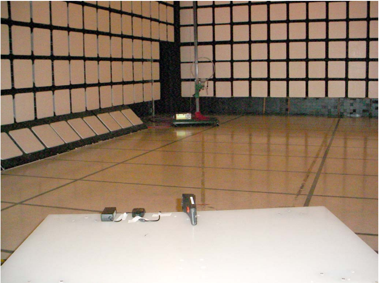
Radiated Emissions @ 10 m – Orthogonal Position 2
