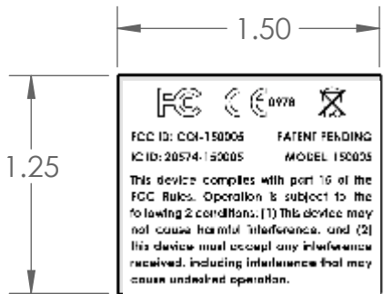
FCC LABEL FOR BUBBLE MAKER SCALE: 1:1
