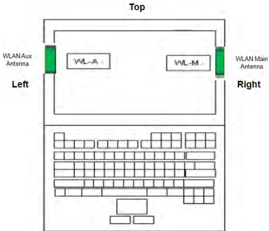
Fig.11 Antenna position of EUT (Front view)
