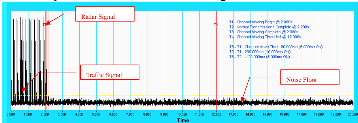
Channel Closing Transmission Time & Channel Move Time ac80 @ CH 106 - 5530 MHz
