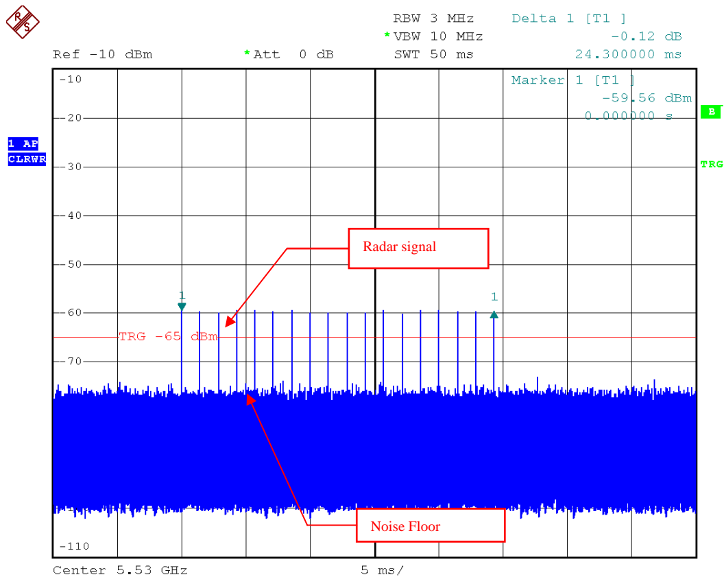
Radar Signal 1
