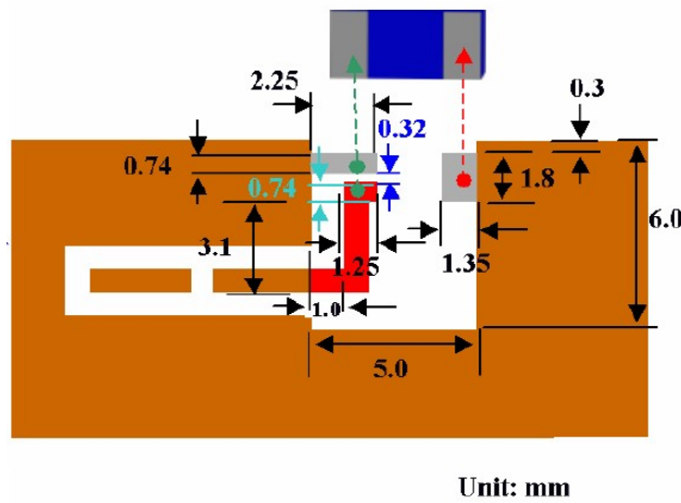
Fig. 2 Outlook and dimension of evaluation board
