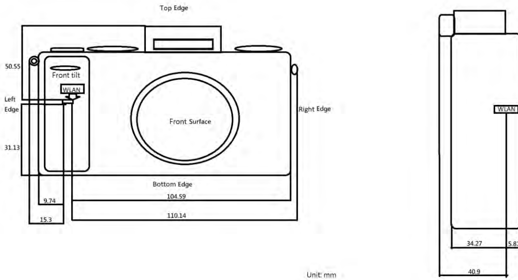
Fig.7 Antenna position
