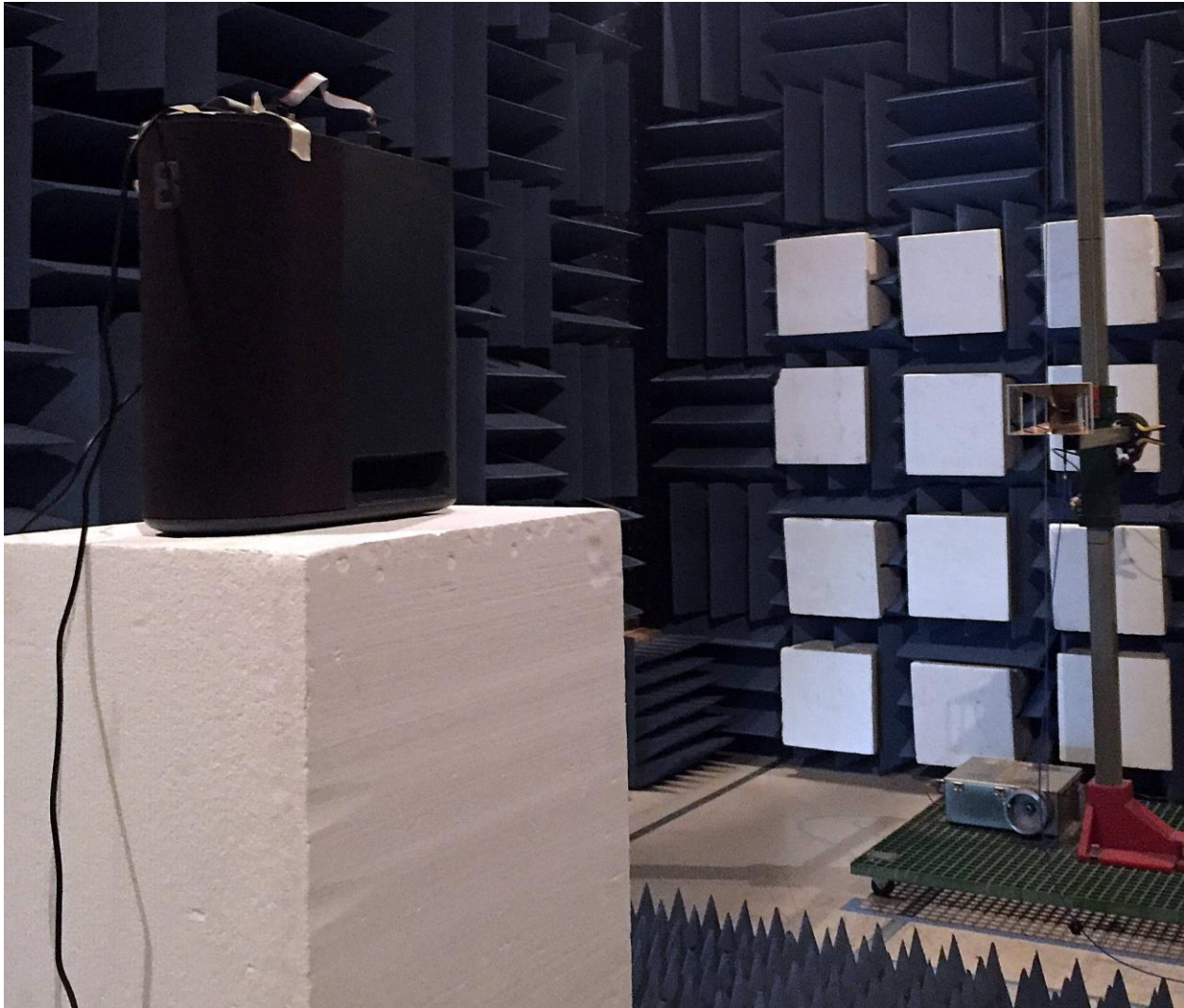
Figure 2: Unwanted Radiated Emissions (1 to 18GHz) Test Setup
