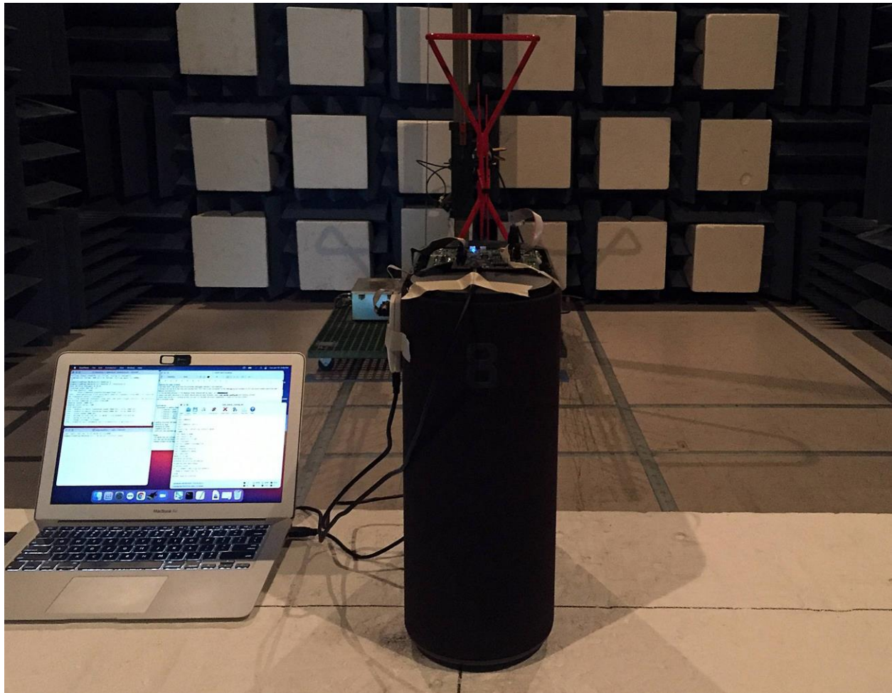
Figure 1: Unwanted Radiated Emissions (30 to 1000MHz) Test Setup
