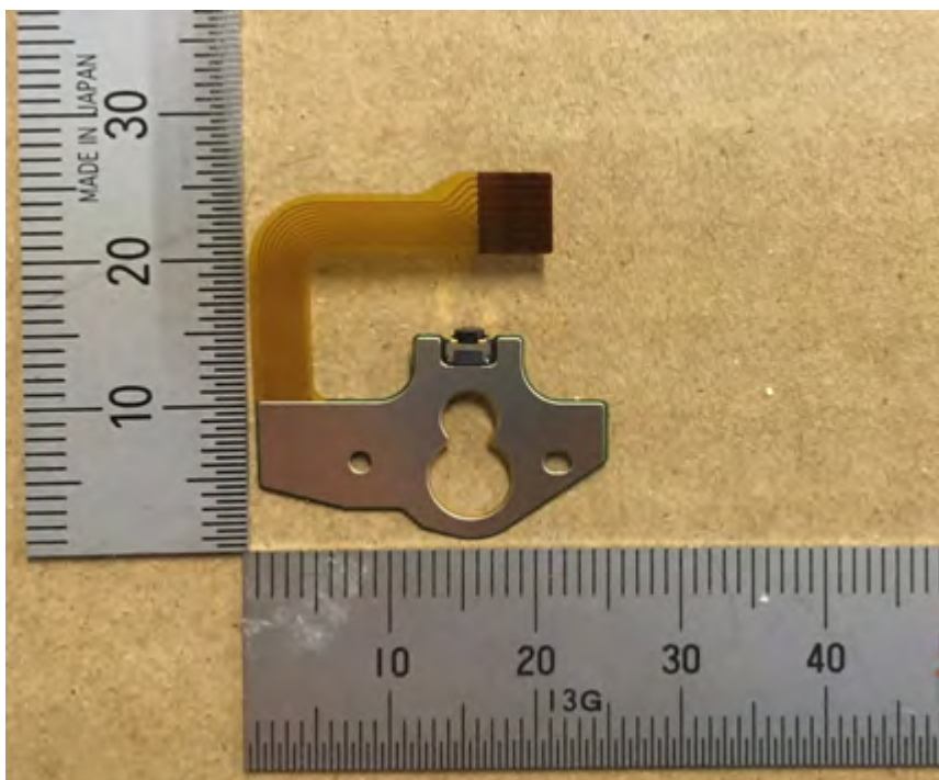
FPC COMMAND_F_B
