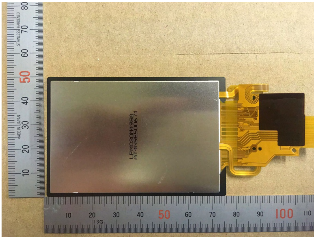
LCD_B
