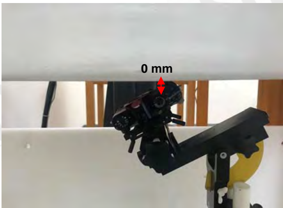
Fig.4 EUT Front tilt side to flat phantom
