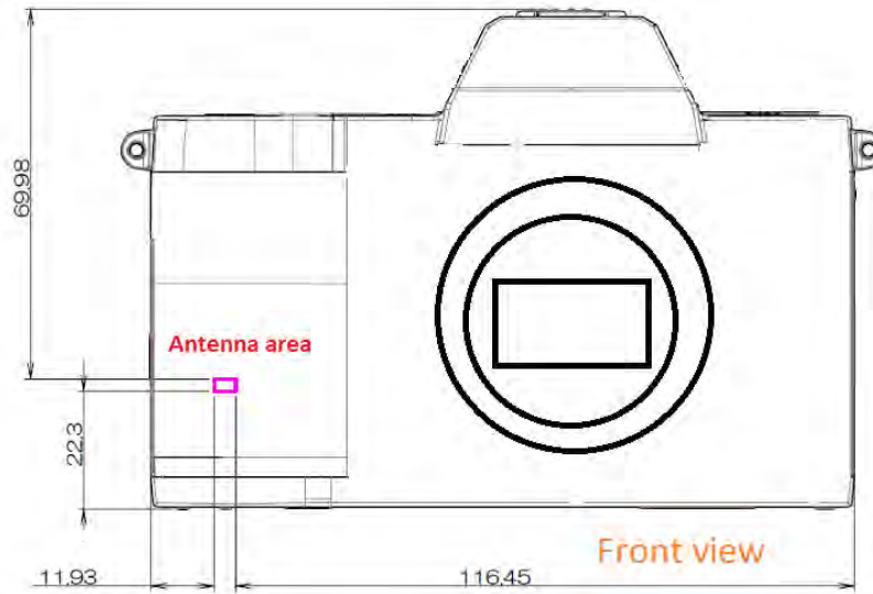
Fig.11 Antenna location
