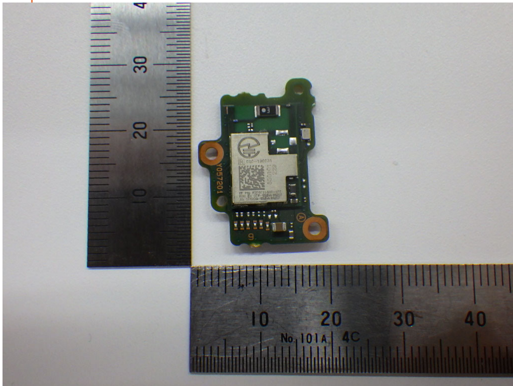
WLAN&BLE Antenna
