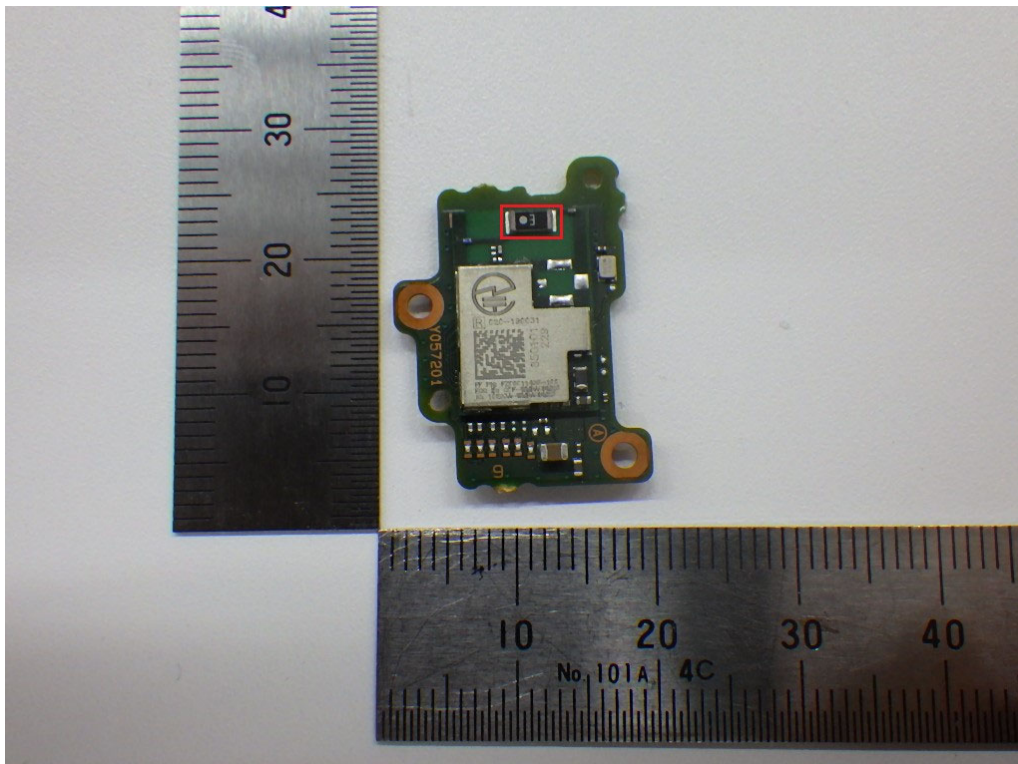
WLAN&BLE Antenna
