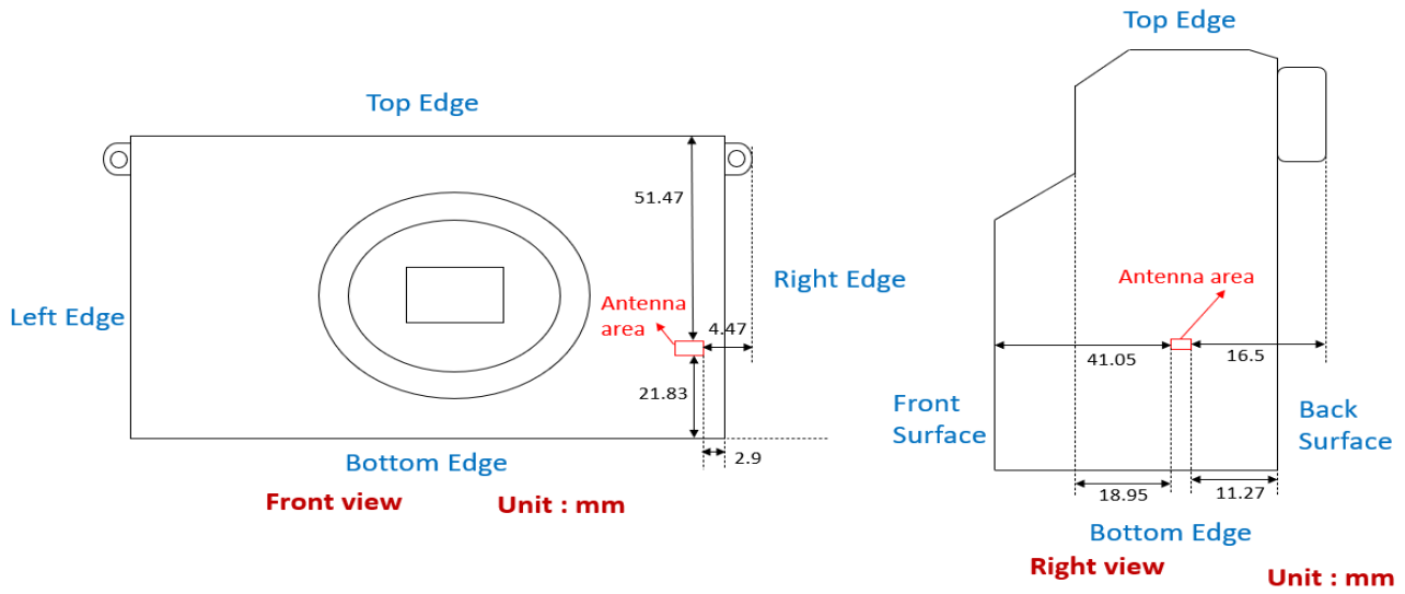
Photograph 5. Antenna position of EUT
