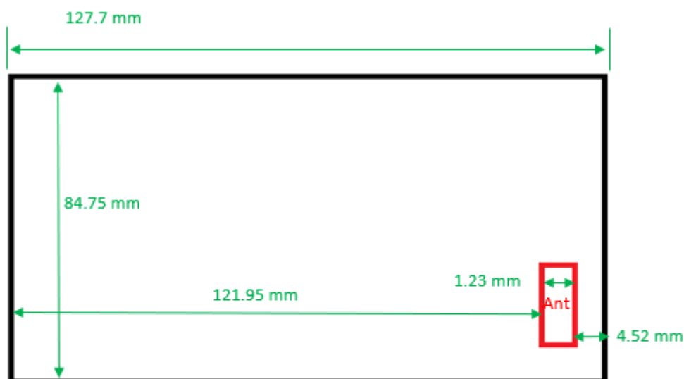
Photograph 9. Antenna position of EUT (Front view)
