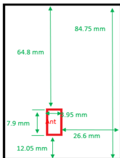
Photograph 10. Antenna position of EUT (Right view)
