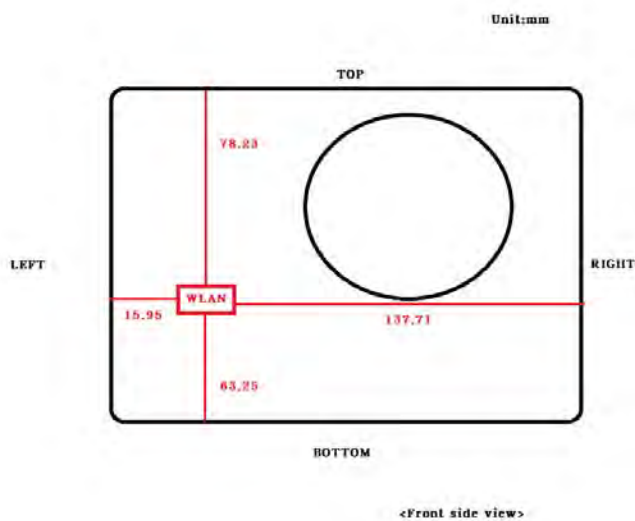
Fig.8 Antenna position (Front side)
