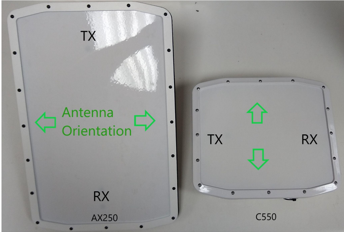
Antenna Orientation comparison of AX250 and C550. AX250 antenna plate is wider and rotated 90 degrees CW.
