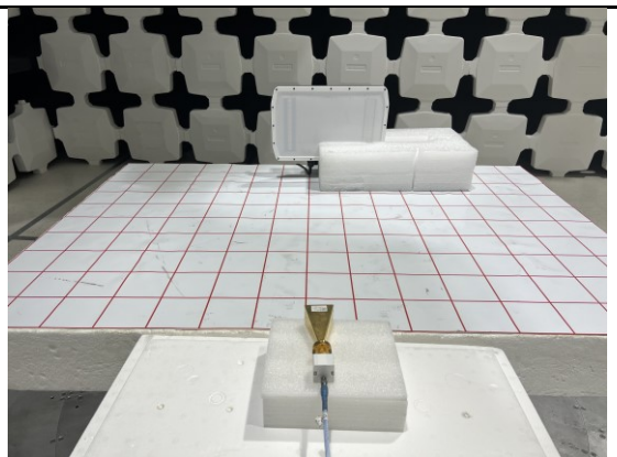
Radiated Emission Test above 40GHz Front view
