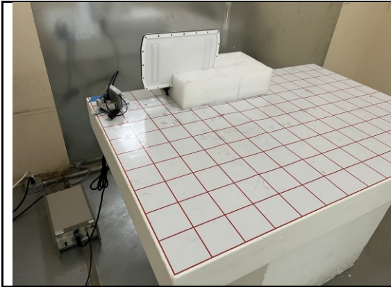
AC Line conducted emission Front View
