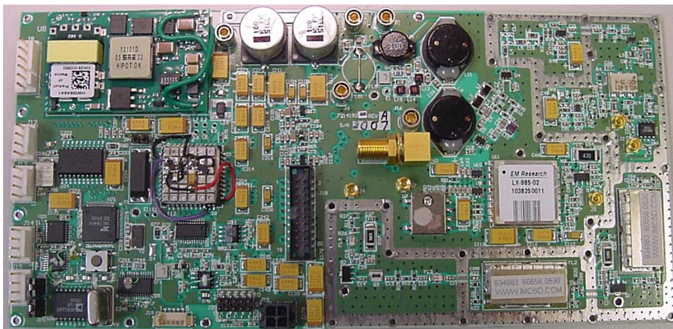
IF Processor Board (IFU) 7214192000
