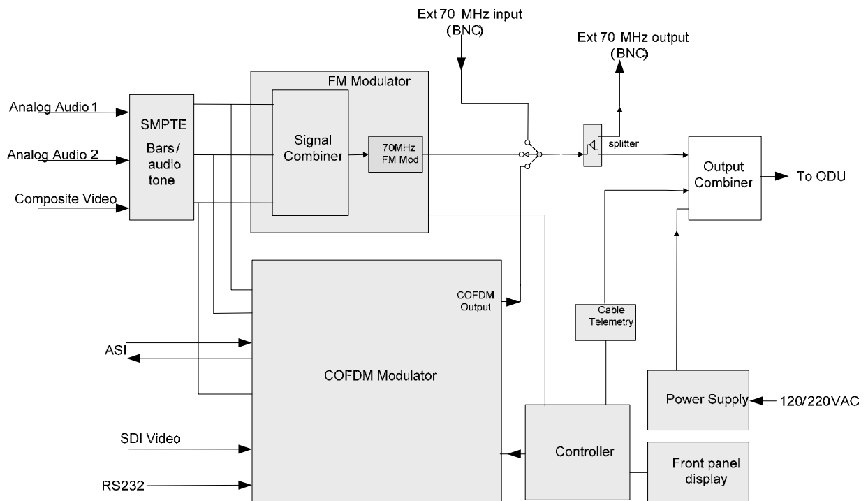
TruckCoder II (Indoor Unit)
