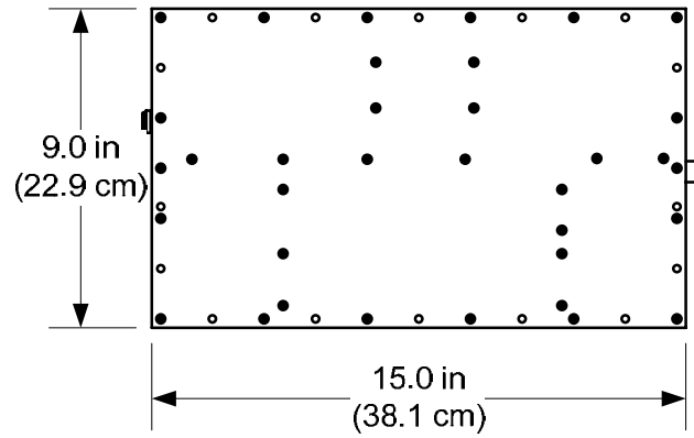
Figure 5 ODU Footprint
