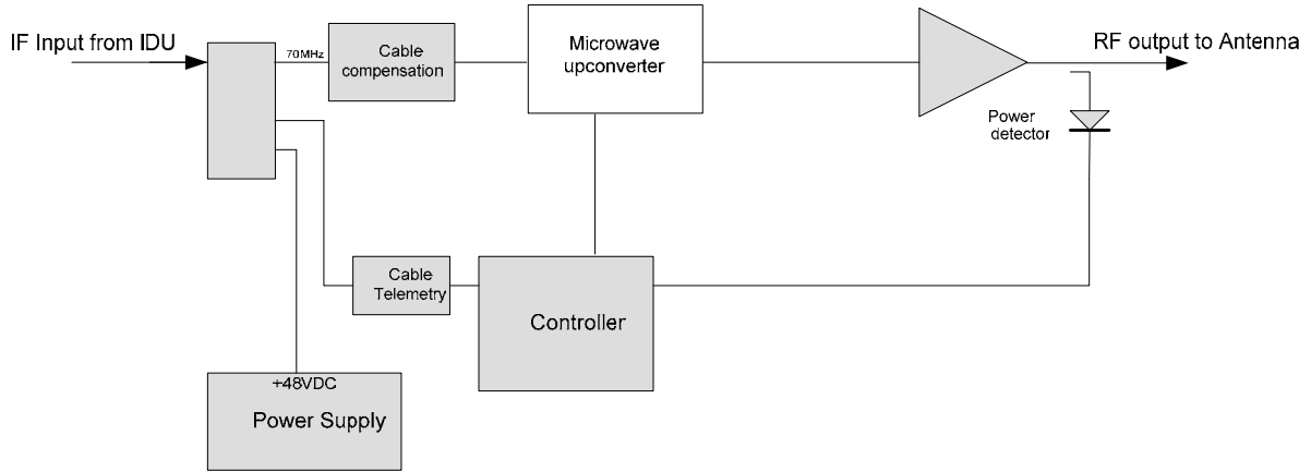
TCII Outdoor Unit
