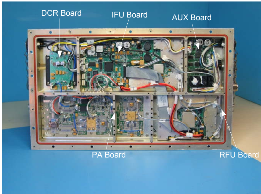
7GHz TCII Outdoor Assembly (ODU) 8014192700
