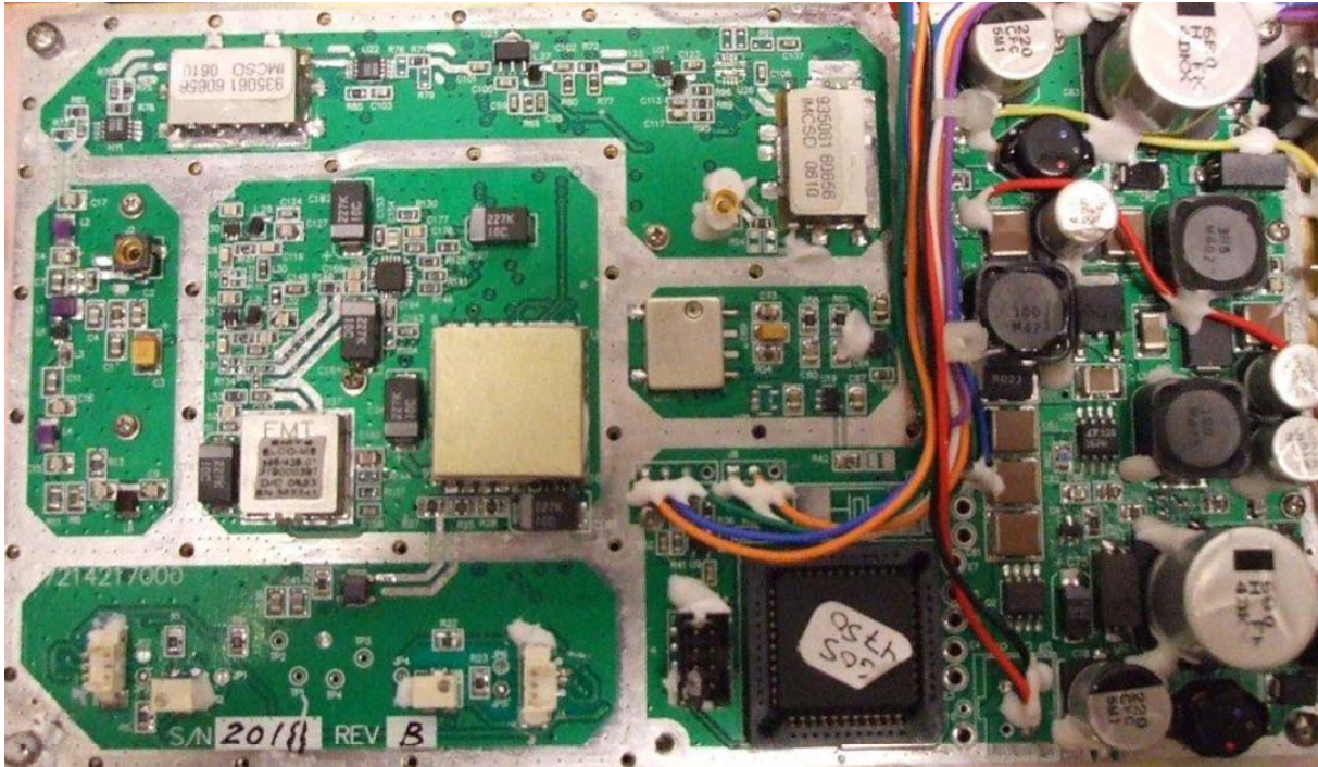
Front View
