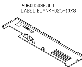
SWITCH COVER
