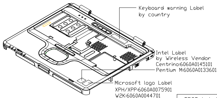
TPCB Label
