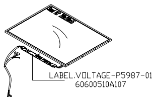
RU_L_PACK_LCM_01_A
