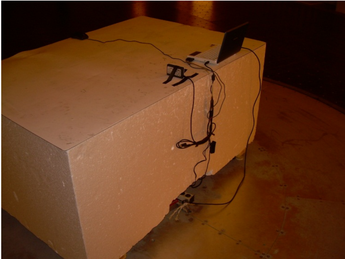
View of Radiated Disturbance – EUT On Edge Placement
