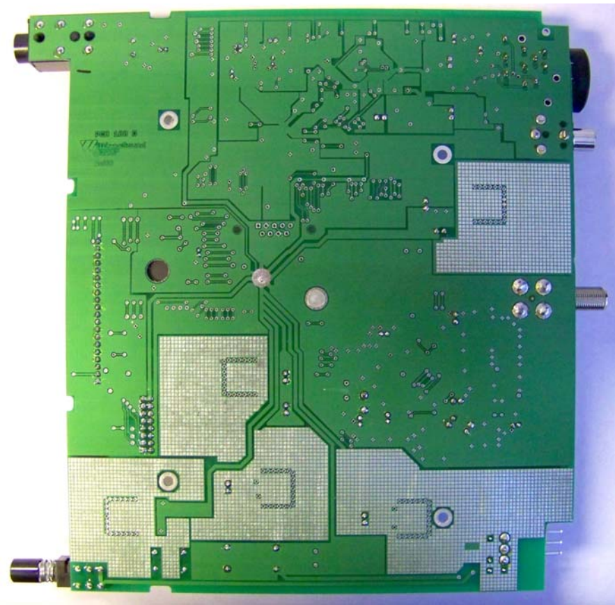
Motherboard Bottom
