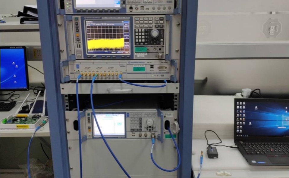
DFS test setup photo
