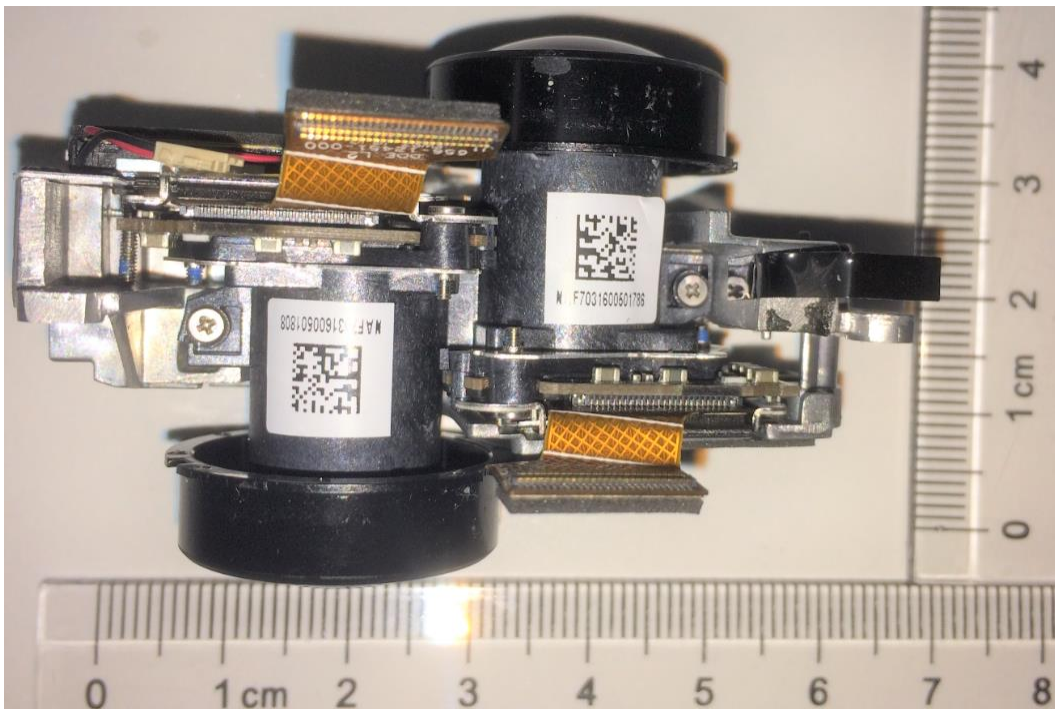
Lens Module-Back
