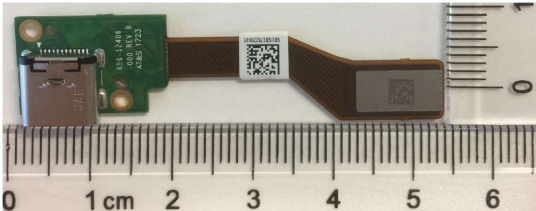
RFPC, USB-Back
