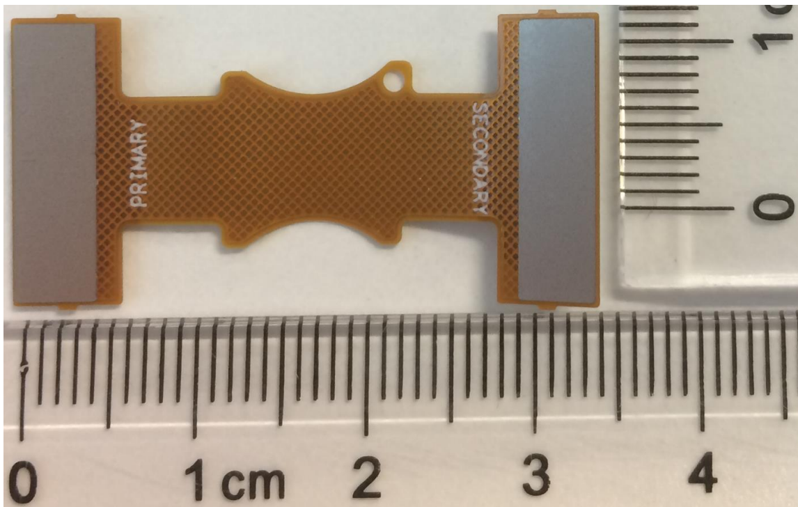
FPC, INTER-PROCESSOR-Back
