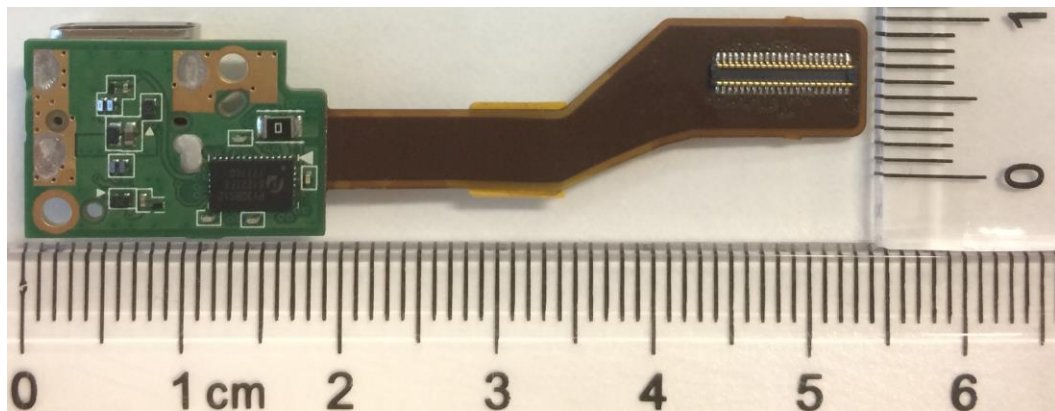
RFPC, USB-Back
