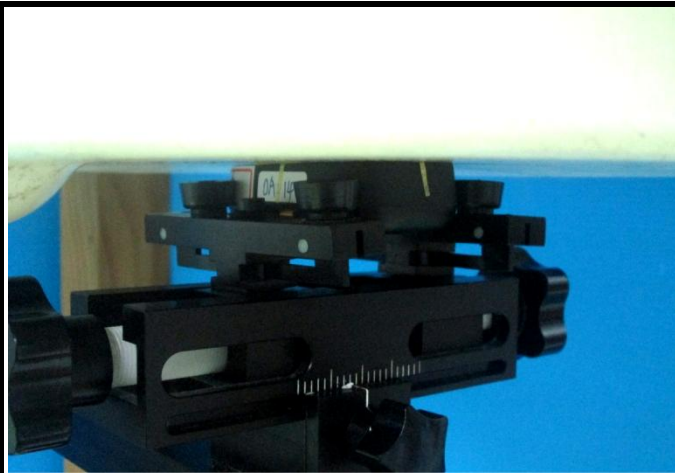
Front Face of EUT with 0 cm Gap
