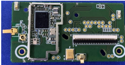
340-31977-000 PCBA, DISPLAY AND SHUTTER-Front with shield removed, CPPM1
