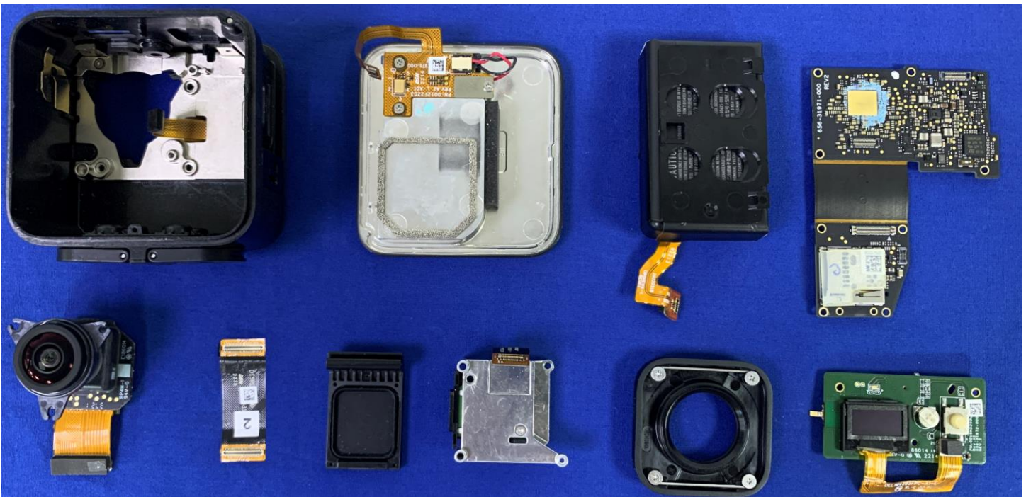
Front/rear cover, Mic, Speaker, battery, Main board, lens module, FPC, I/O door, USB board, lens cover, Shutter/display board removed, CPPM1
