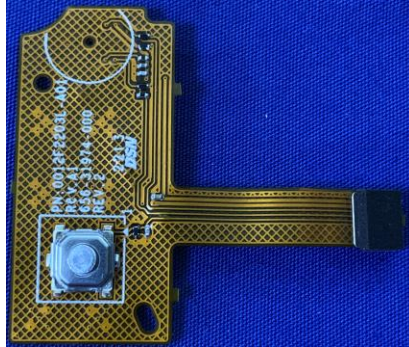
340-31974-000 ASSY, FPC, FRONT MIC AND MODE, CPPM1
