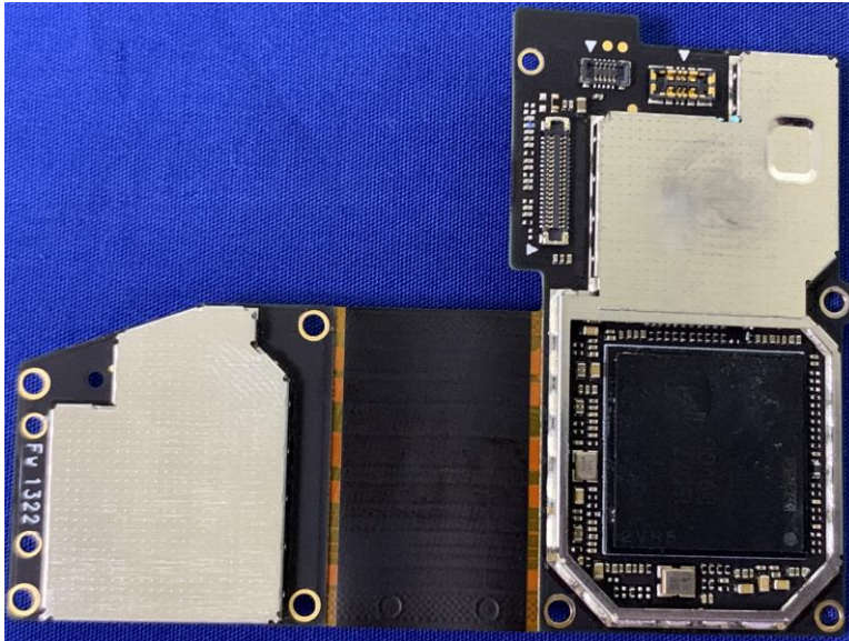
340-31976-000 RFPCA, MAIN-Front with shield, CPPM1
