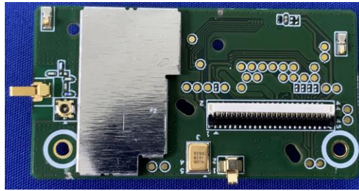
340-31977-000 PCBA, DISPLAY AND SHUTTER-Front with shield, CPPM1
