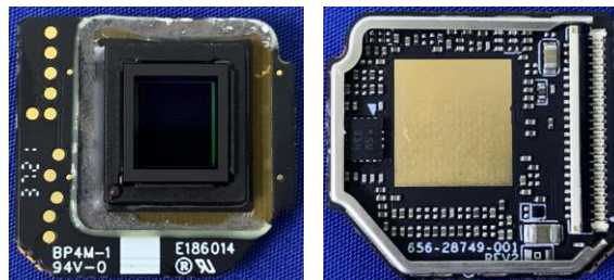
340-28748-001 PCBA, SENSOR BOARD, CPPM1
