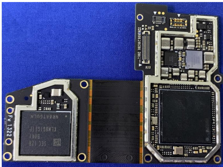
340-31976-000 RFPCA, MAIN-Front with shield removed, CPPM1
