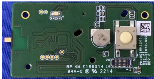
340-31977-000 PCBA, DISPLAY AND SHUTTER-Back, CPPM1
