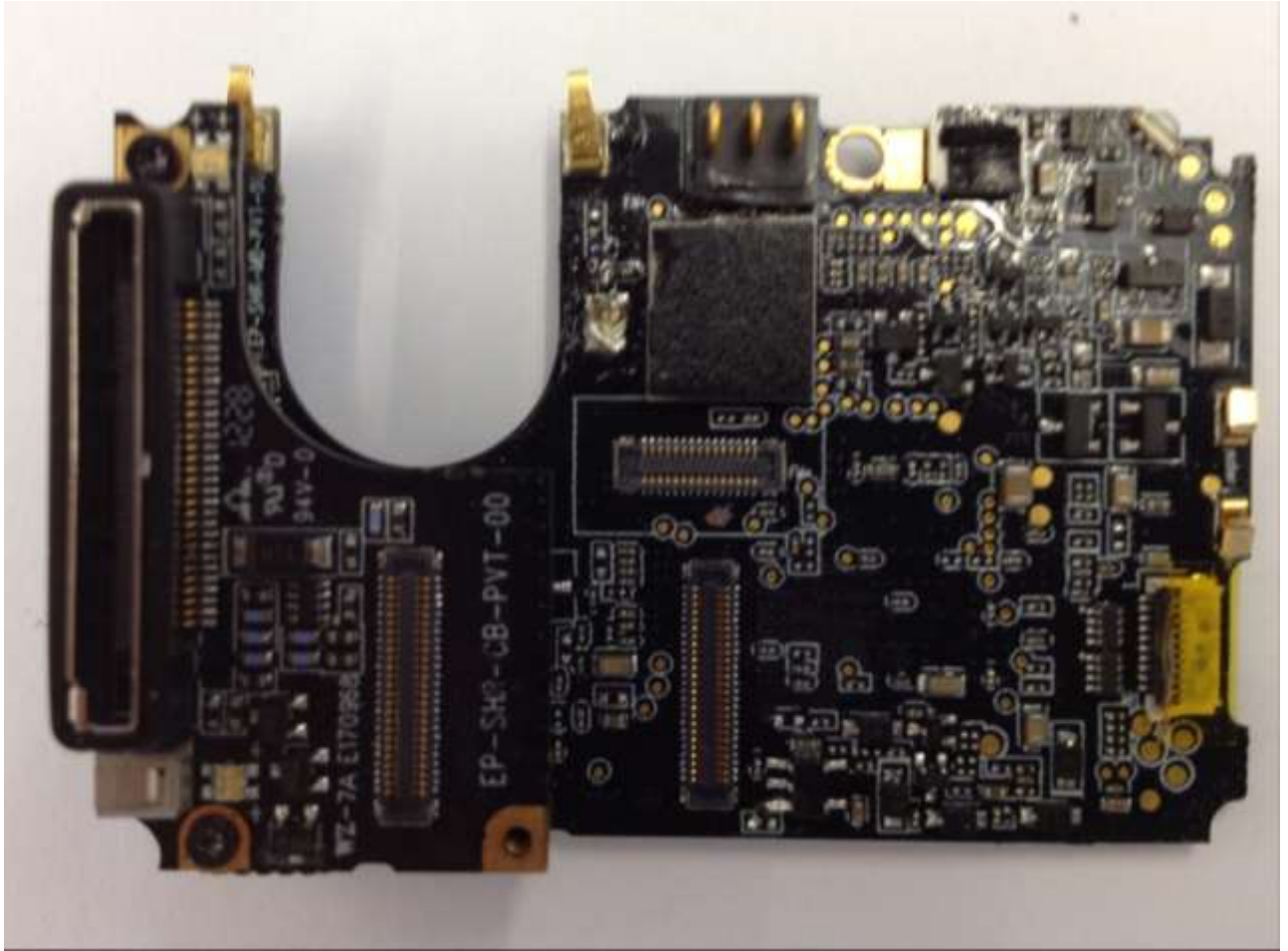
Camera unit and Sensor Board removed from main board
