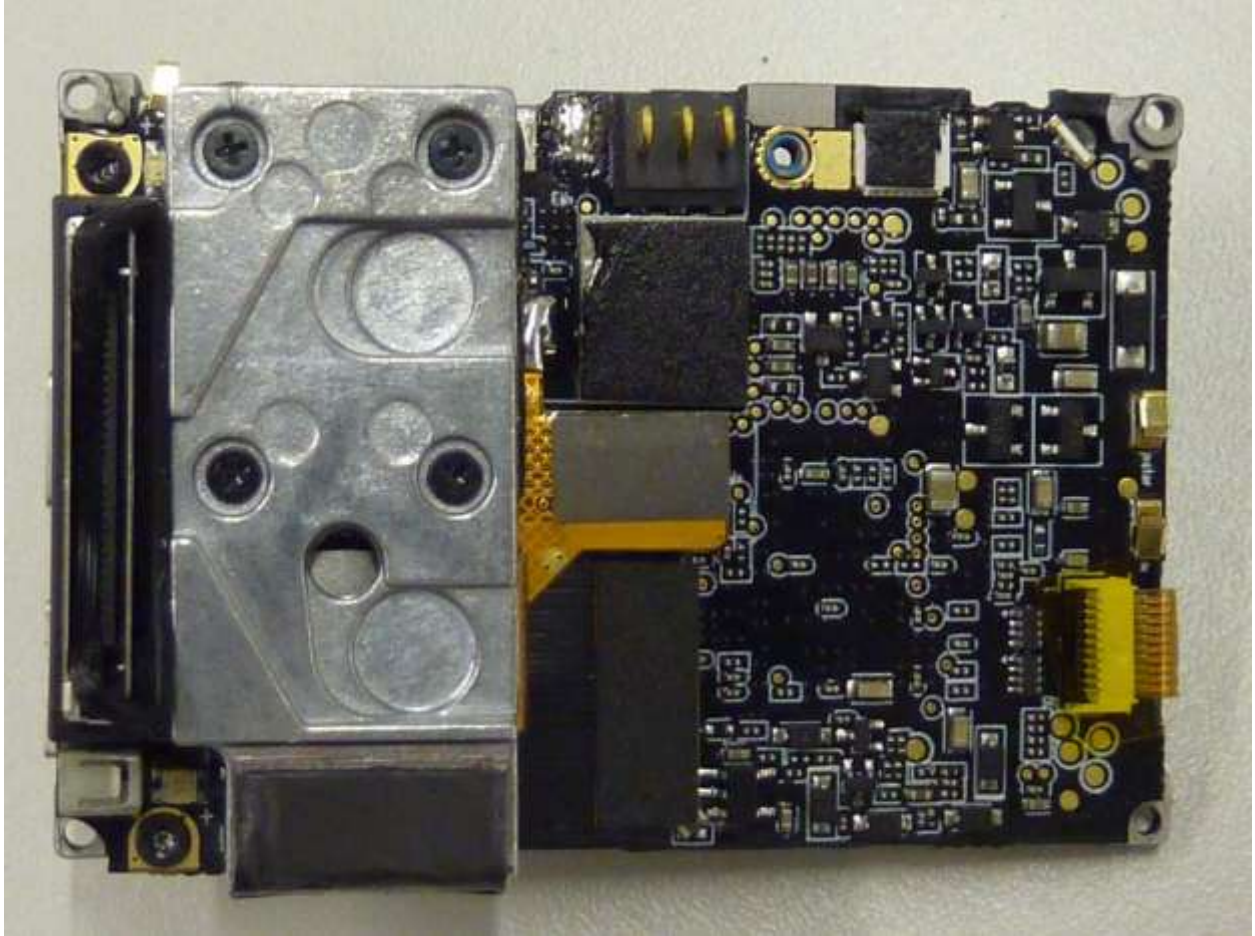
Main Board Back side with Camera unit
