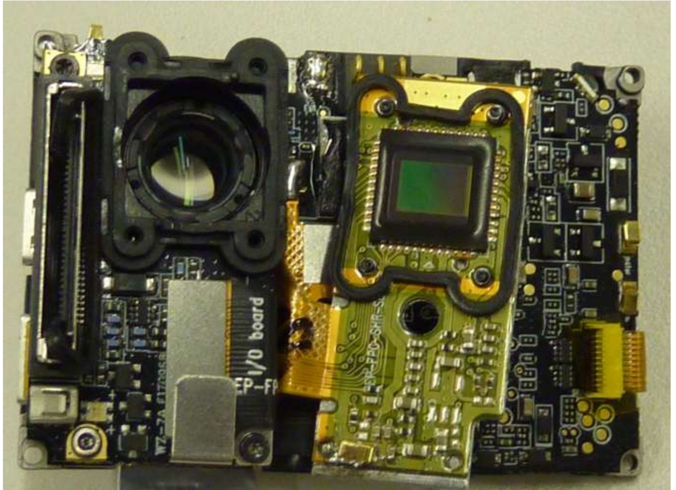
Camera unit and inner side of Sensor Board Exposed
