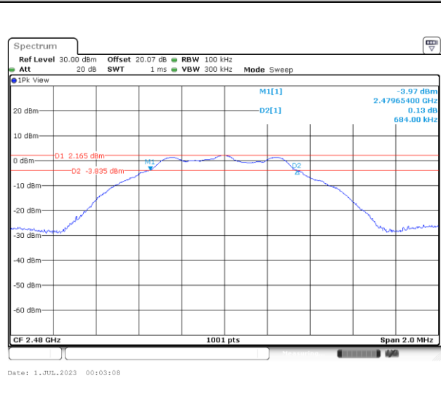
6 dB Bandwidth Plot on Channel 39
