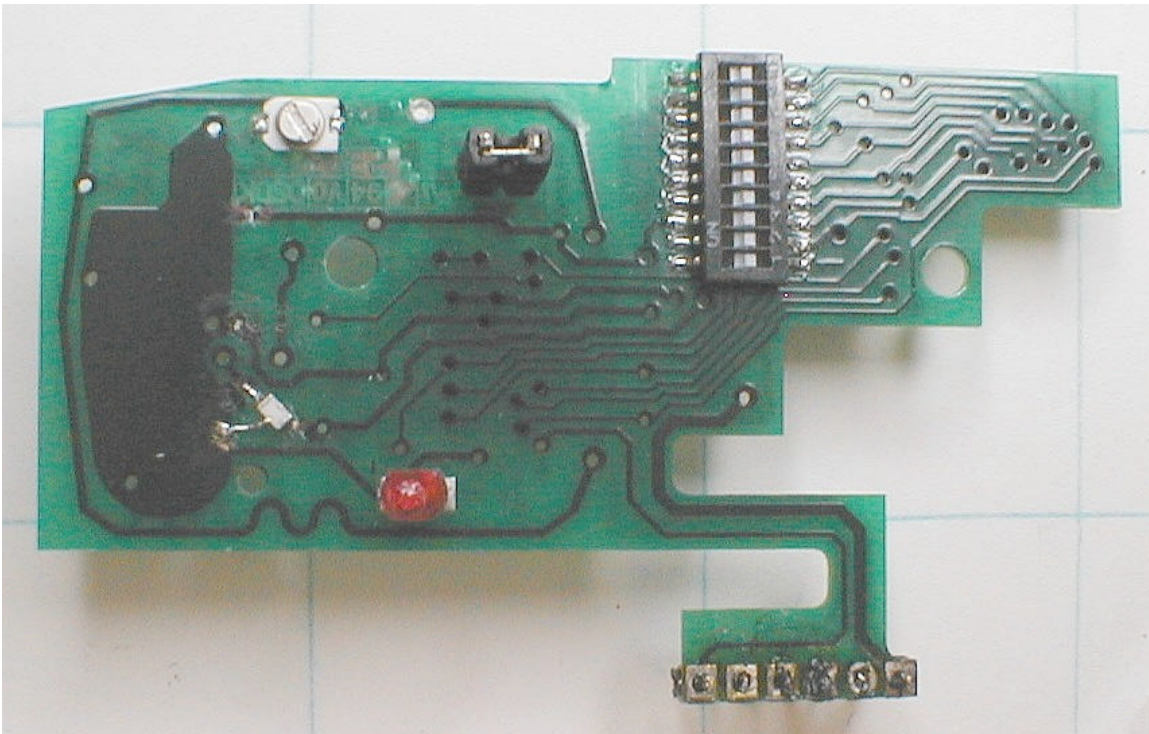
PCB 2 Top View
