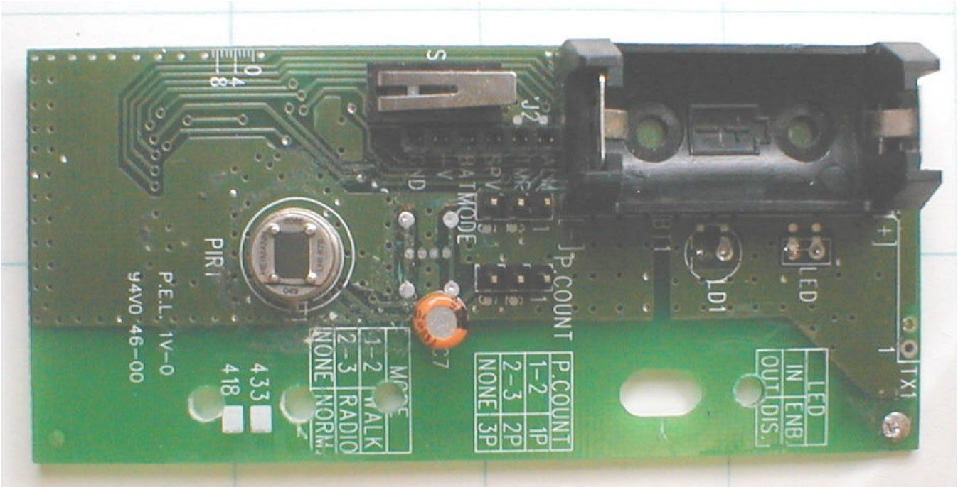
Top View, PCB 2 Removed
