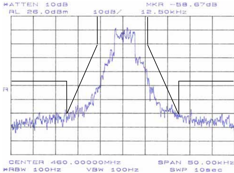
Figure 1. Occupied Bandwidth
