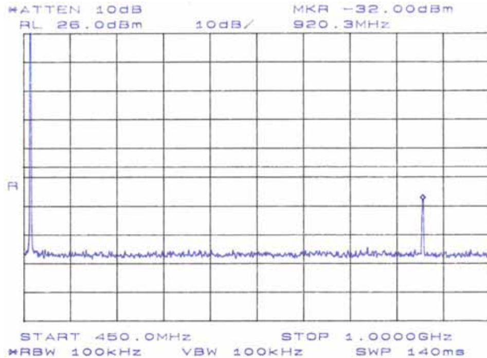
Figure 3. Conducted Spurious Emissions, 450 – 1000MHz
