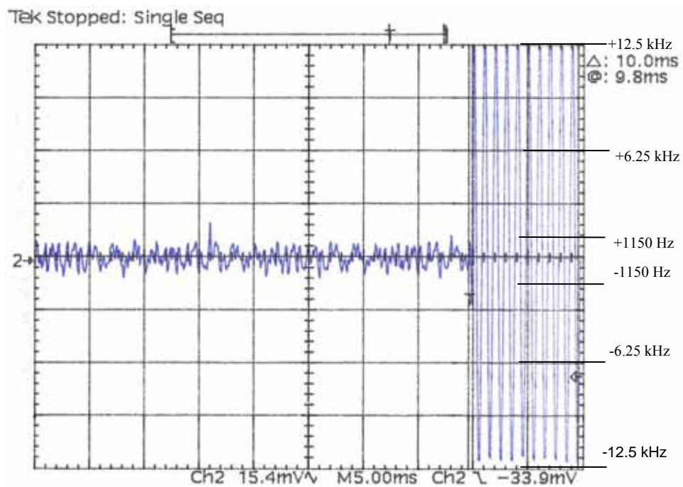
Figure 7. Transient Frequency Behavior, Turn-Off Without Modulation
