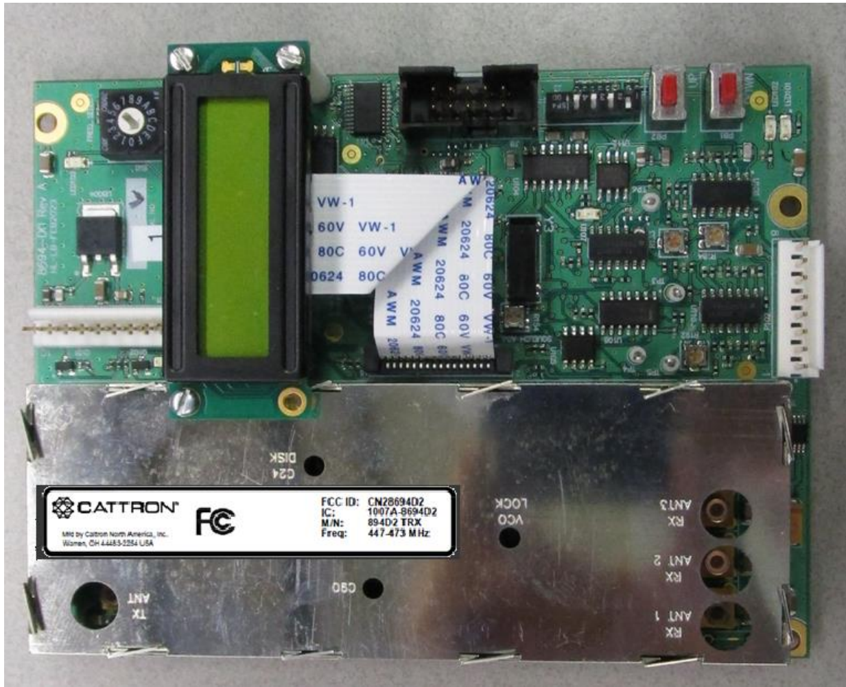
UNIT TOP VIEW WITH RF SHIELD and FCC/IC information label
