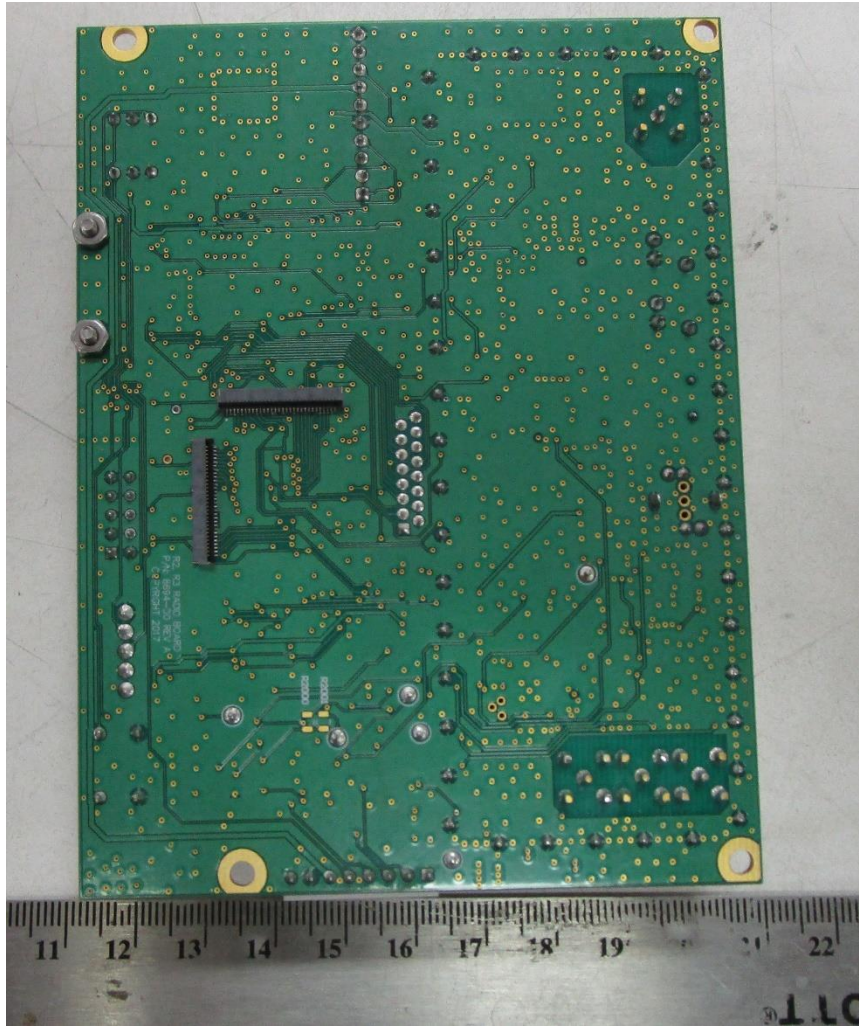
BOTTOM view
