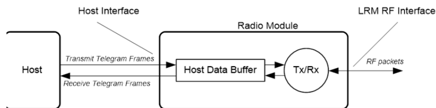
Figure 2.2 - Data communication model
