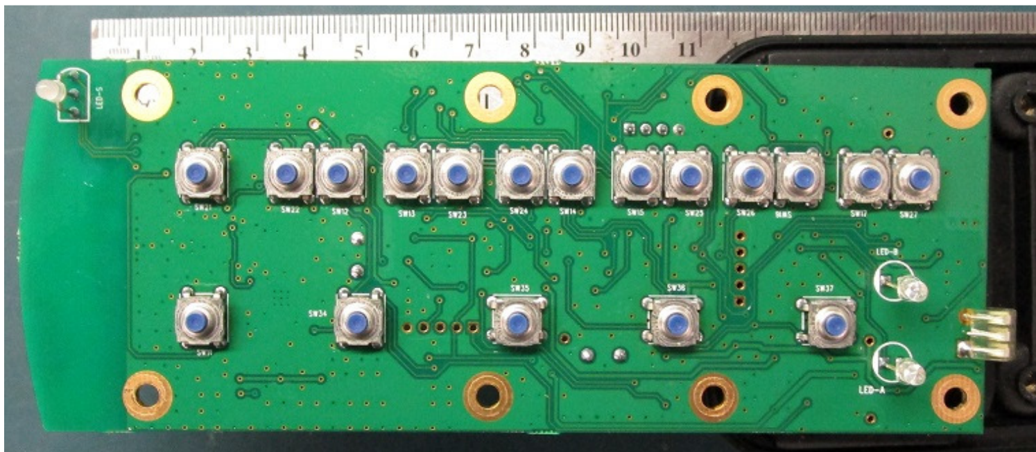
TOP View
