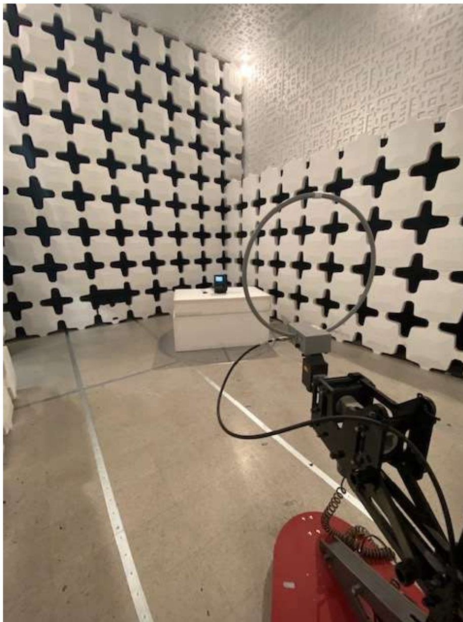
Figure 2. Radiated Emissions Test Configuration (below 30 MHz)
