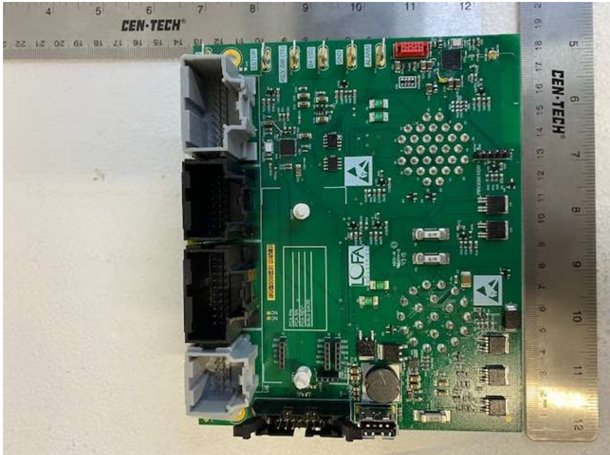
Figure 3. PCB, Top
