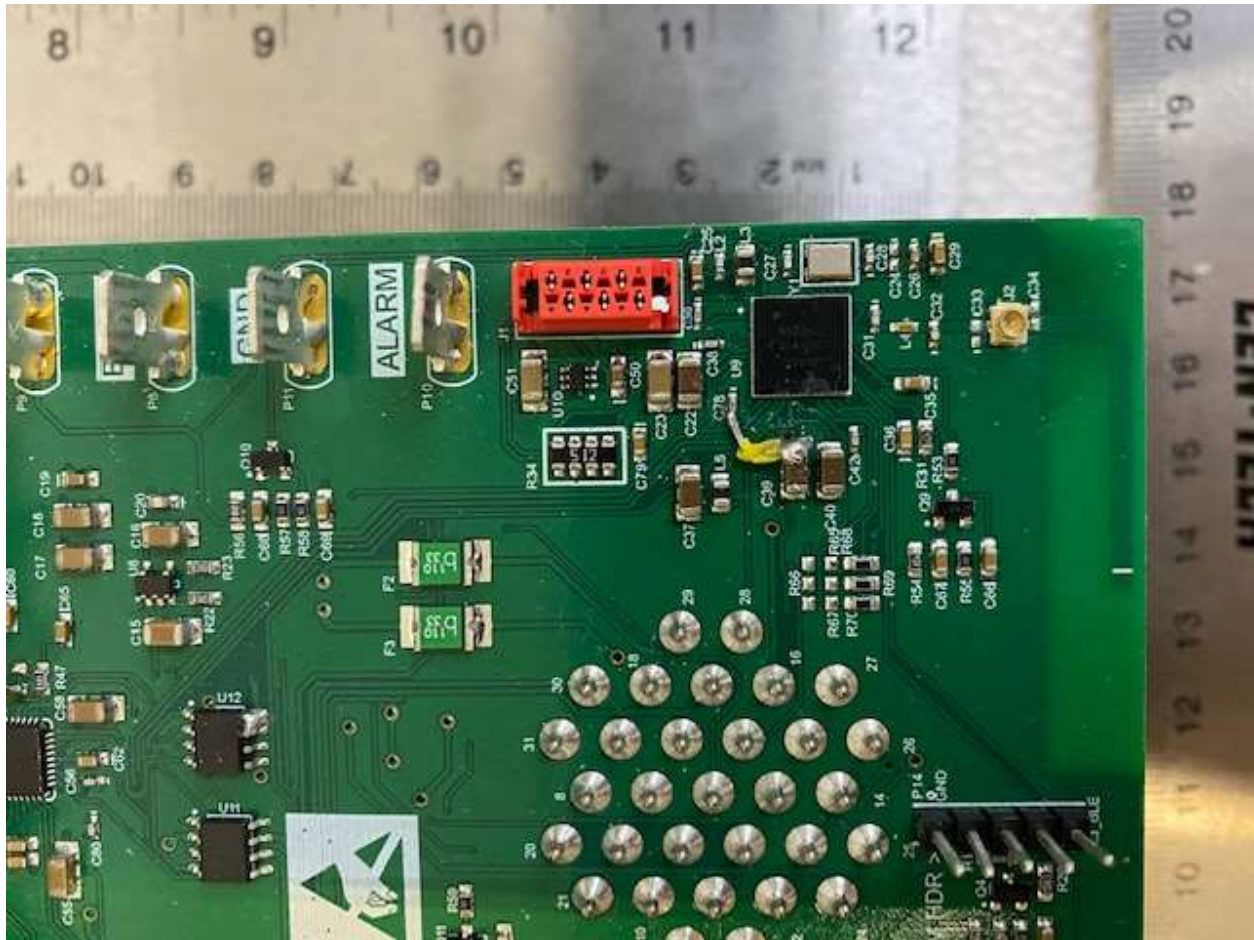
Figure 5. PCB, Close up of BLE
