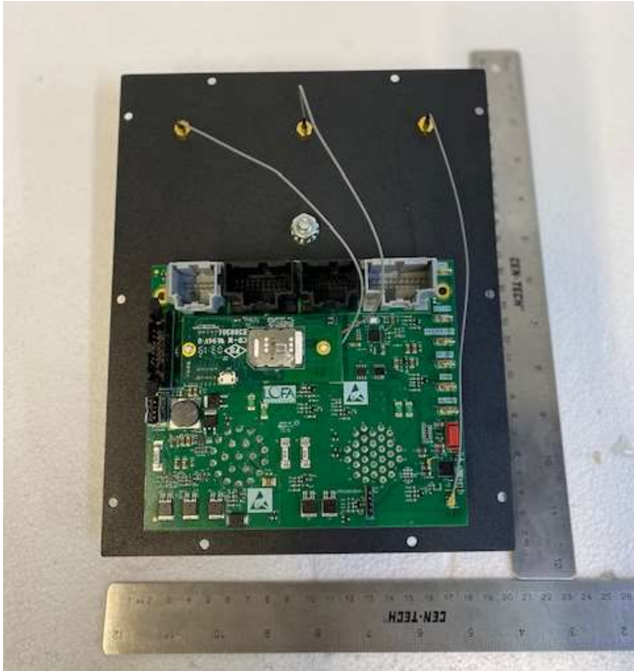
Figure 2. PCB Mounted on Back Panel
