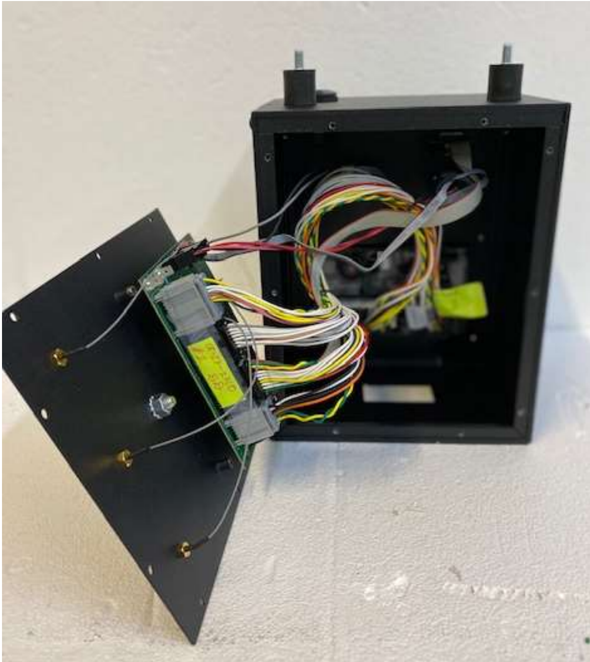
Figure 1. EUT, Back Panel Open, Inside Exposed
