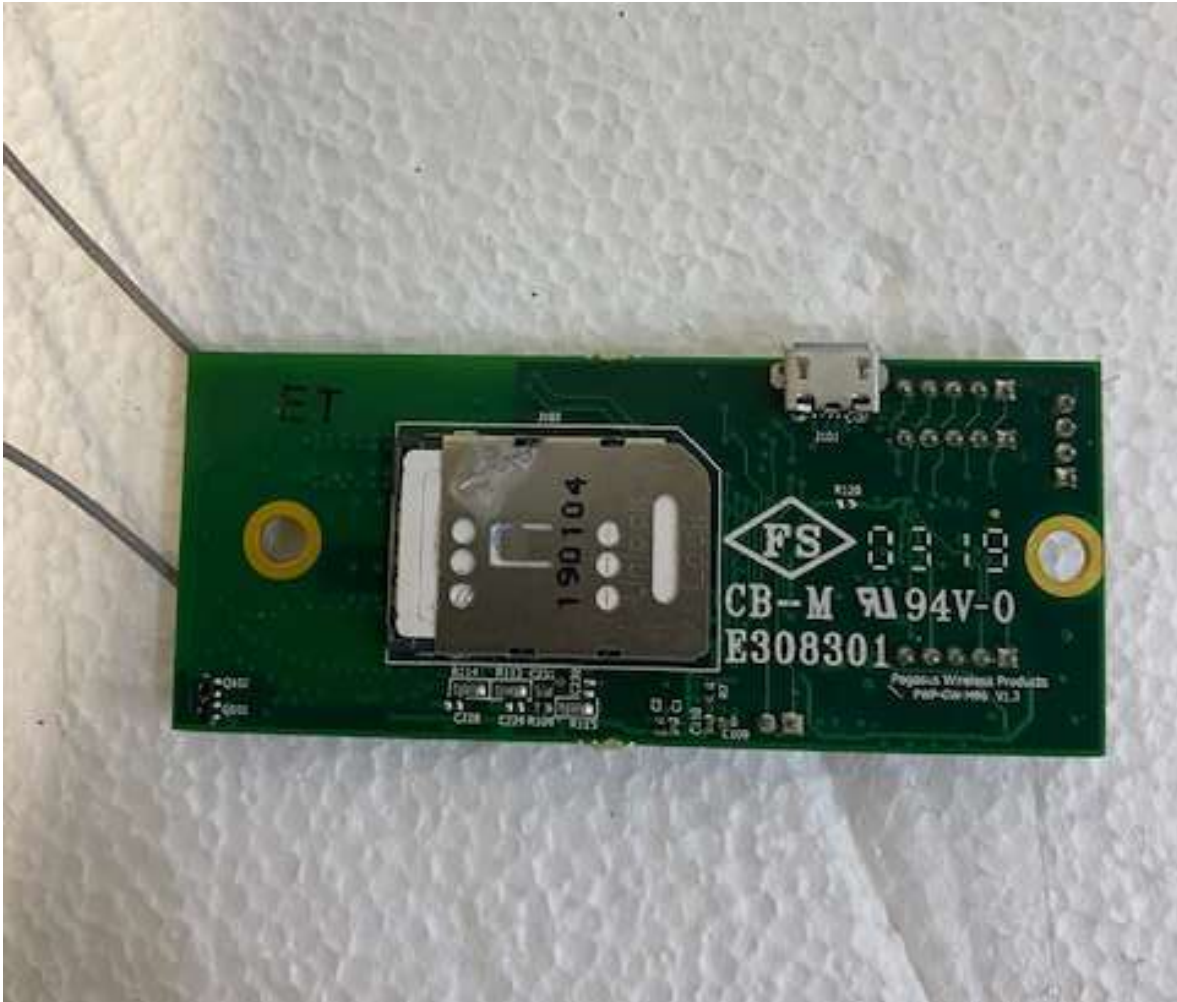
Figure 7. Cell Module, Back
