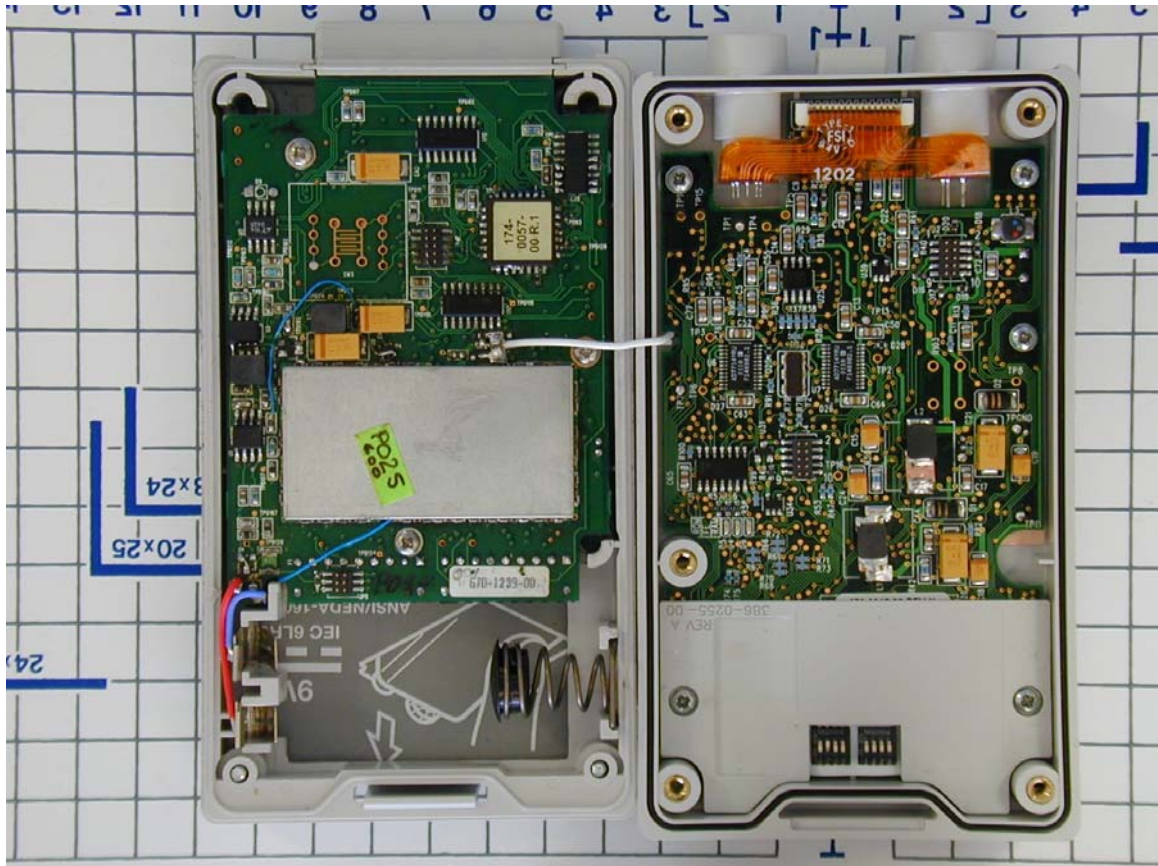
Interior View of 600-1400 MHz MPT
