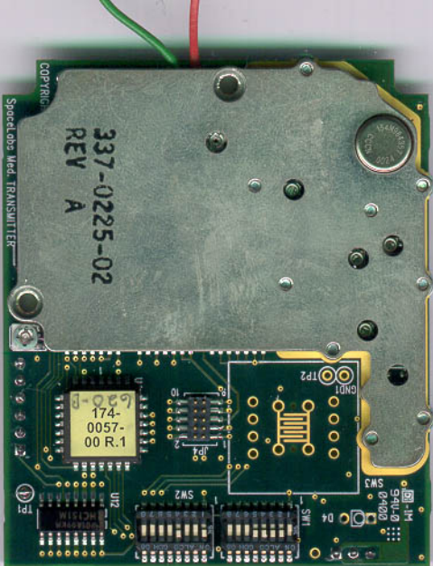
RF Board with Large Shield Installed
