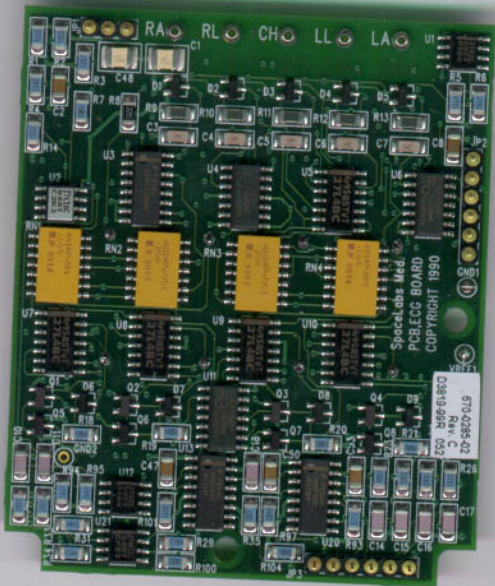
ECG Board
