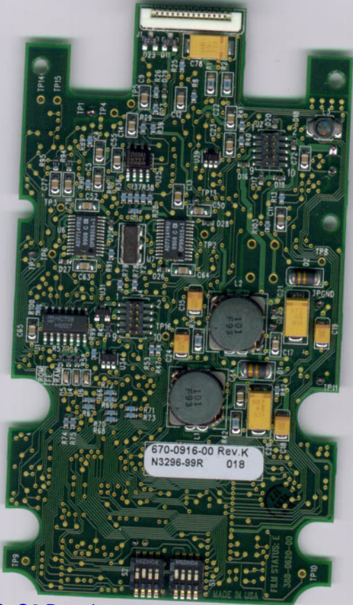
SpO2 Board
