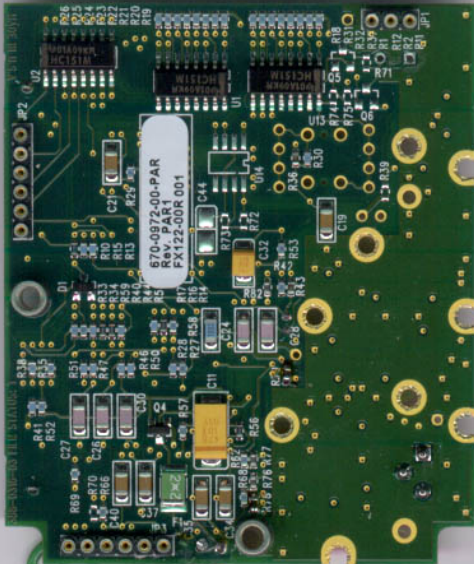
RF Board
