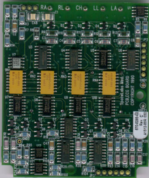
ECG Board
