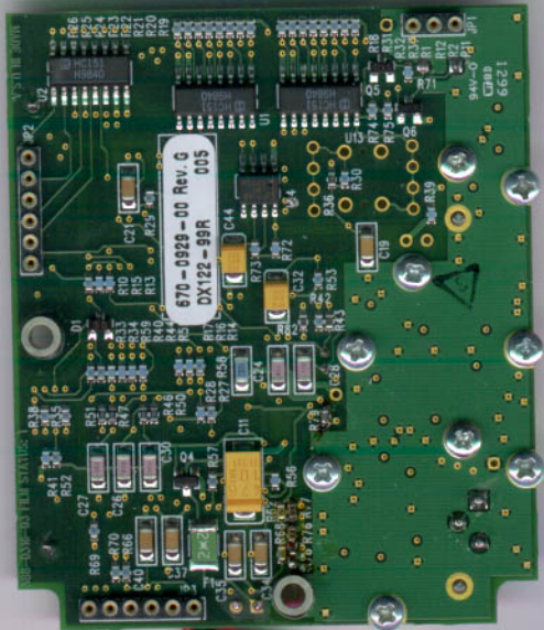
RF Board
