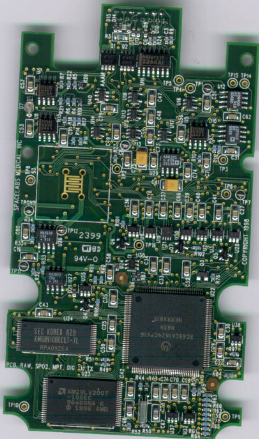
SpO2 Board
