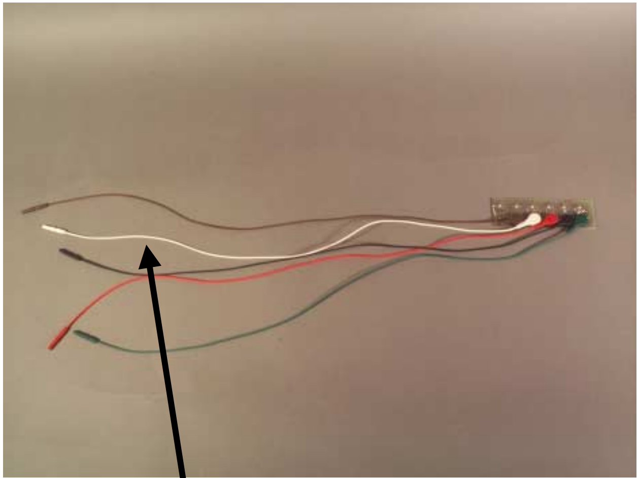
Patient RA ECG Lead acts as the Antenna
