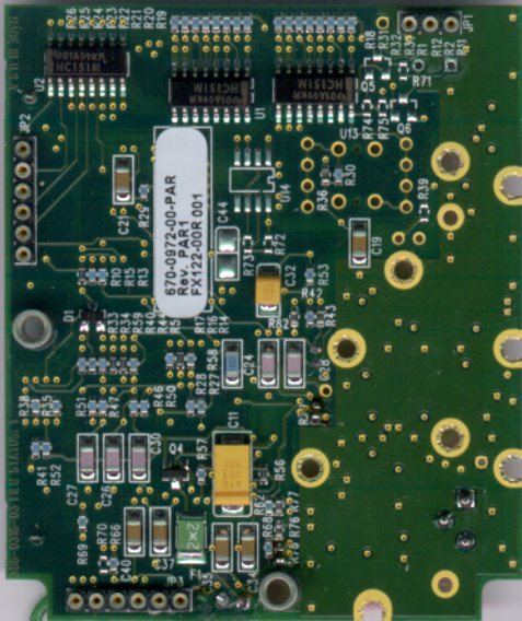
RF Board
