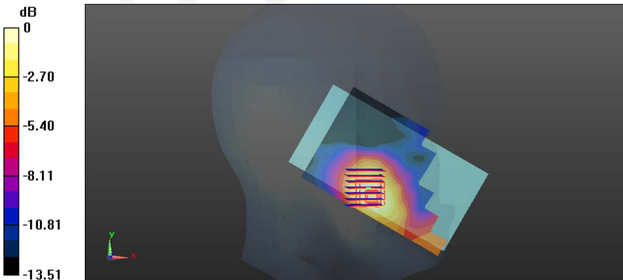
0 dB = 0.151 W/kg = -8.21 dBW/kg
