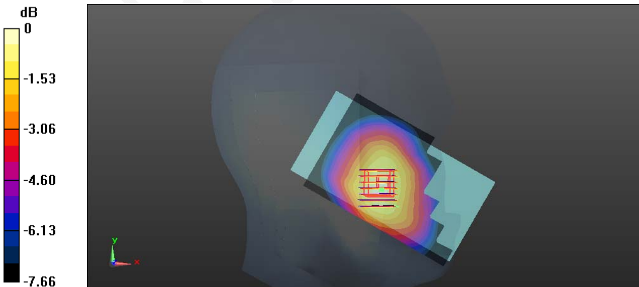
0 dB = 0.191 W/kg = -7.19 dBW/kg
