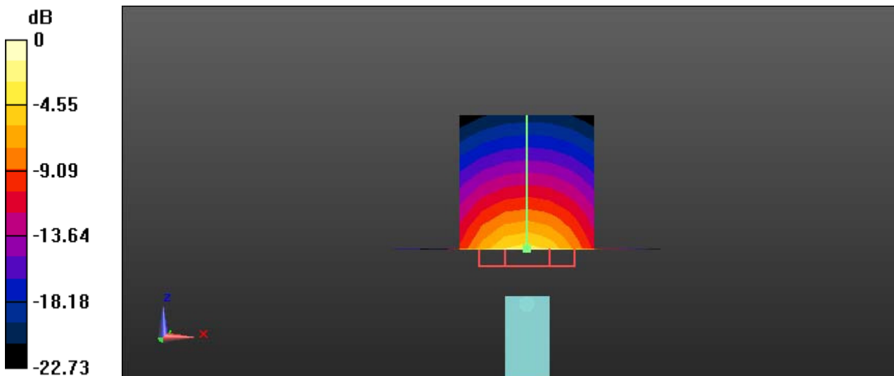
0 dB = 64.9 W/kg = 18.12 dBW/kg
