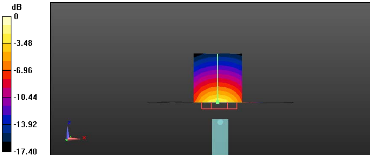
0 dB = 44.2 W/kg = 16.45 dBW/kg
