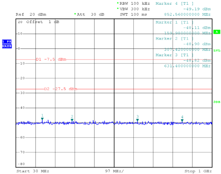
Channel = 9, 30MHz to 1GHz
