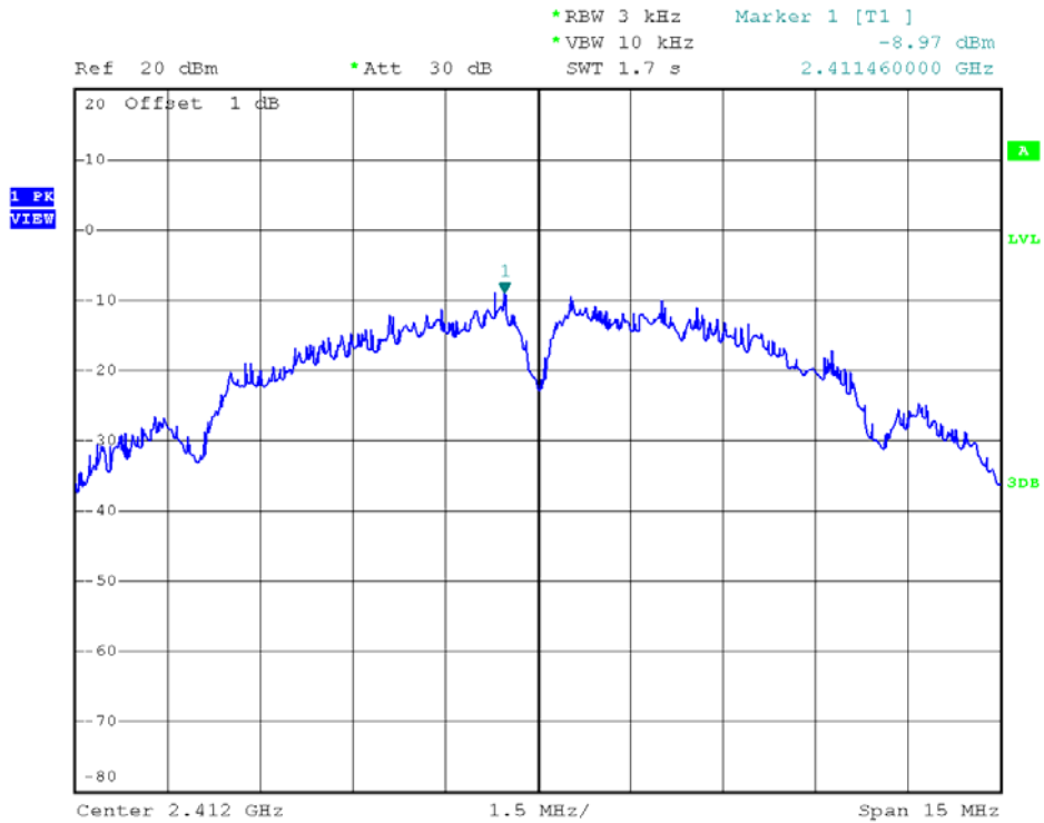
802.11b - Channel 1
