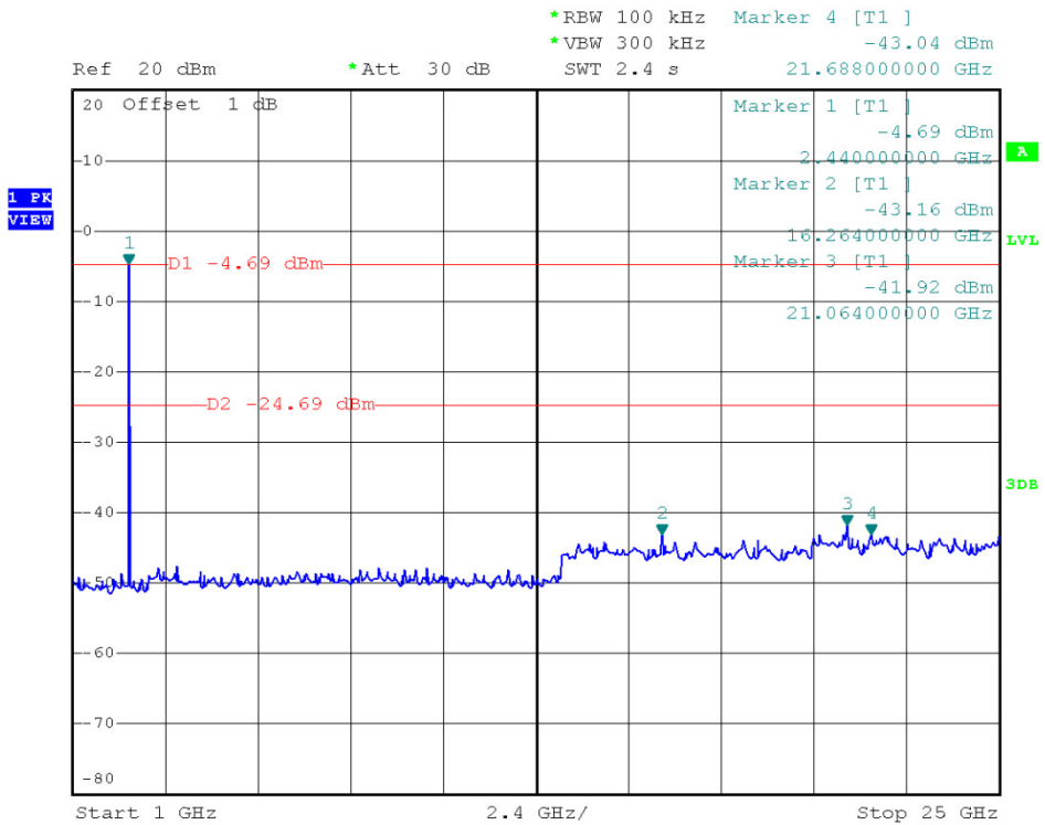
Channel = 19, 1GHz to 25GHz
