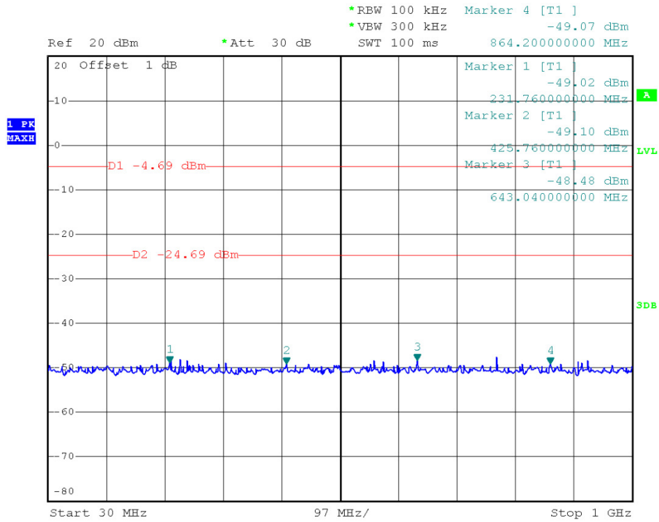
Channel = 19, 30MHz to 1GHz
