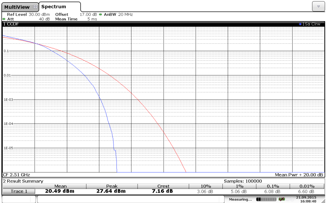
(Plot C1: Band 7/20MHz/16QAM in Ch.20850 1RB Size )
