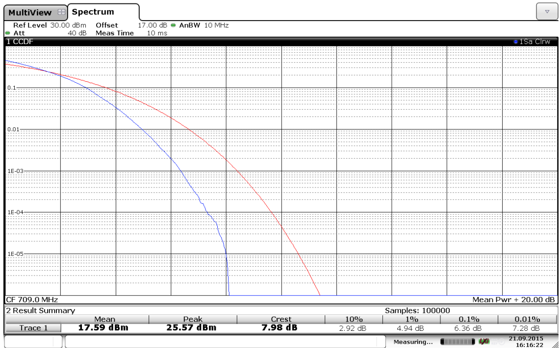
(Plot D1: Band 17/10MHz/16QAM in Ch.23780 1RB Size )
