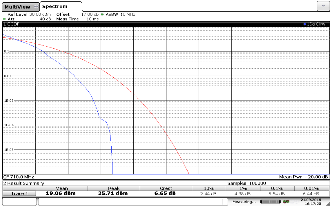
(Plot D3: Band 17/10MHz/16QAM in Ch.23790 1RB Size)
