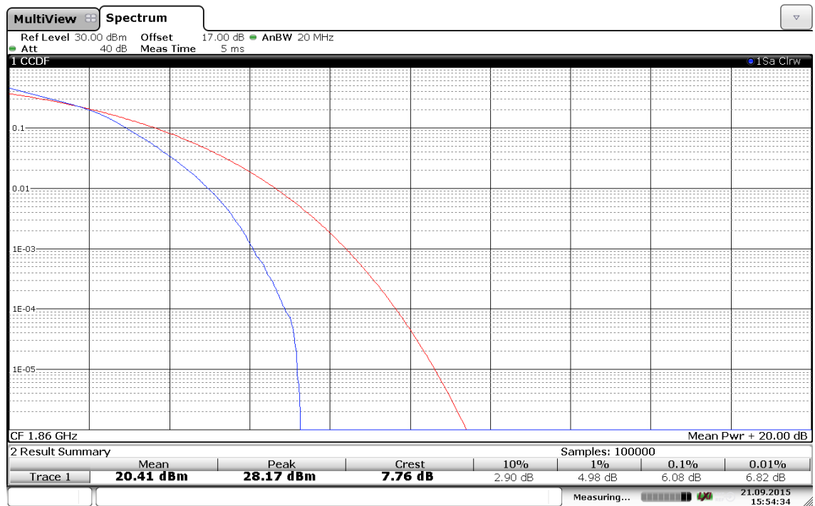
(Plot A2: Band 2/20MHz/16QAM in Ch. 18700 100RB Size)
