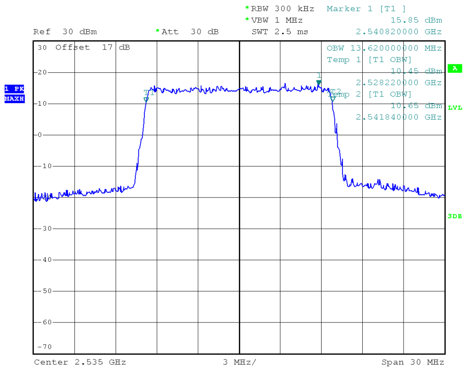
(Plot O1: 99% Occupied Bandwidth LTE Band 7/15MHz/QPSK)
