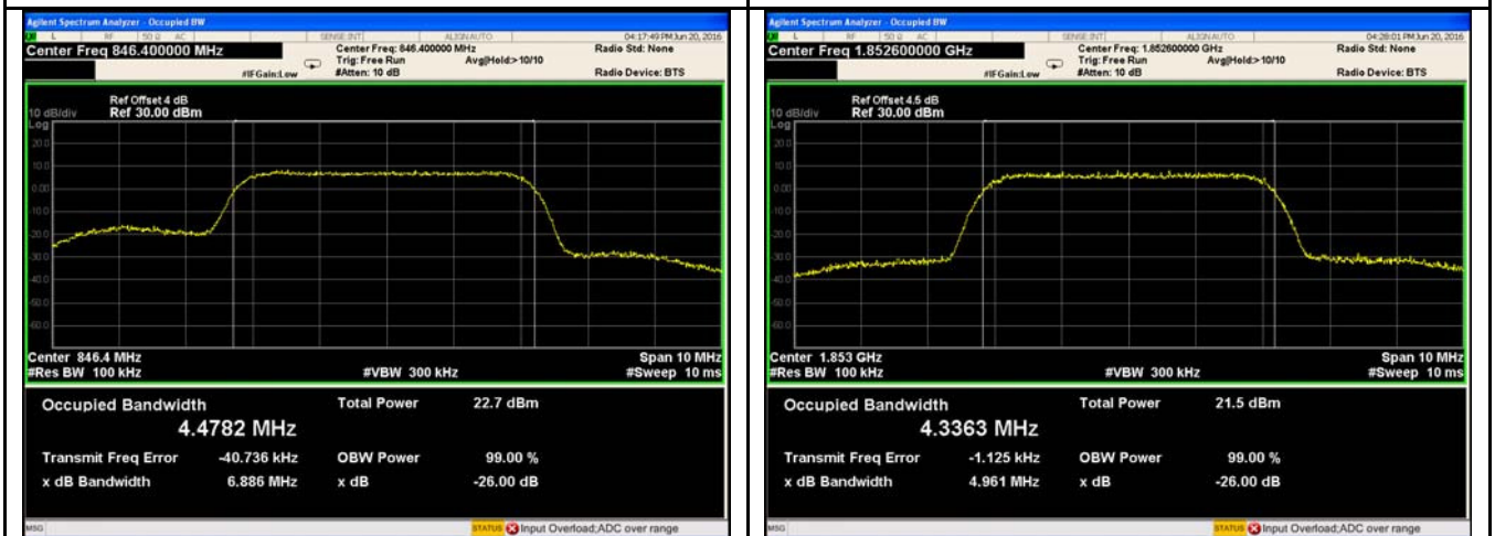
Band V BW - High CH 846.4 MHz
