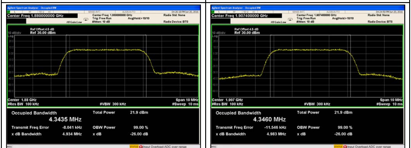
Band II BW - Mid CH 1880MHz
