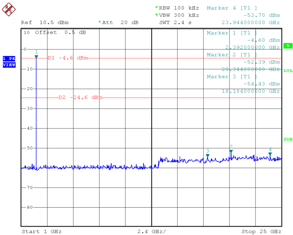
(Plot A.2: Channel = 0, 1GHz to 25GHz)
